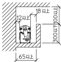
床面取付時(上下可動)
