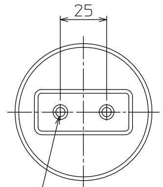
2-木ねじ用穴
